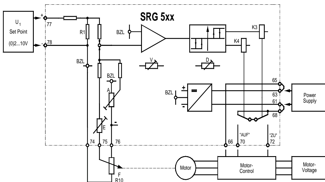
Fig.2: Basic circuit diagram
