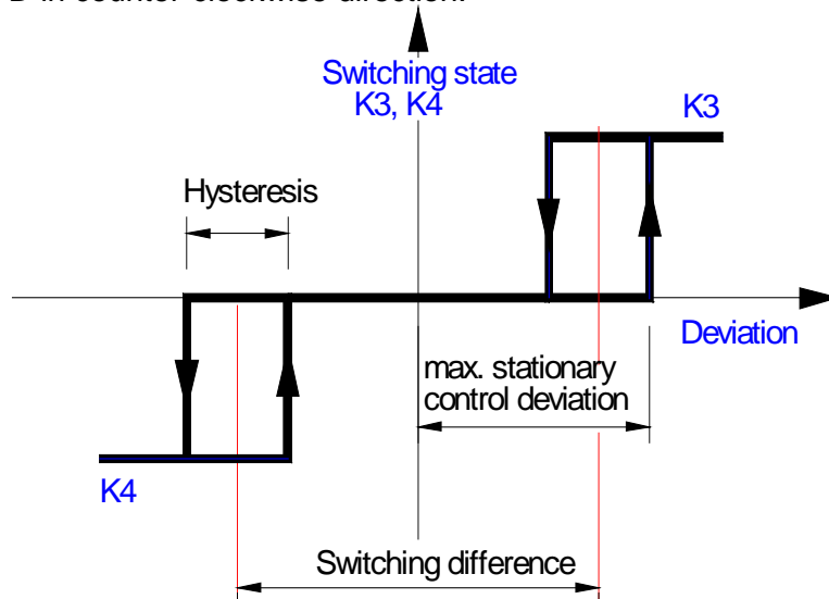
Fig.5: Switchpoints of 3-point controller
