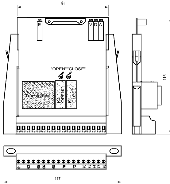
Fig.4: SRG5x1
